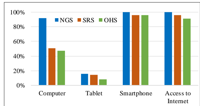
Figure 2 Percentage of teachers owning electronic devices and access to the Internet by school type
