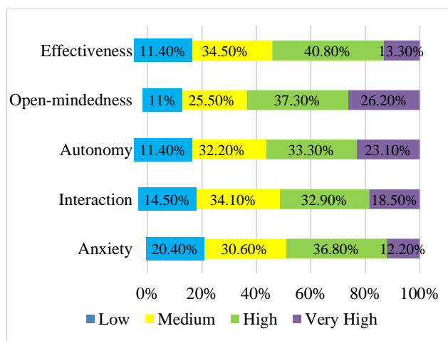
Figure 1: Four levels of the five constructs of students' attitude towards online English learning
